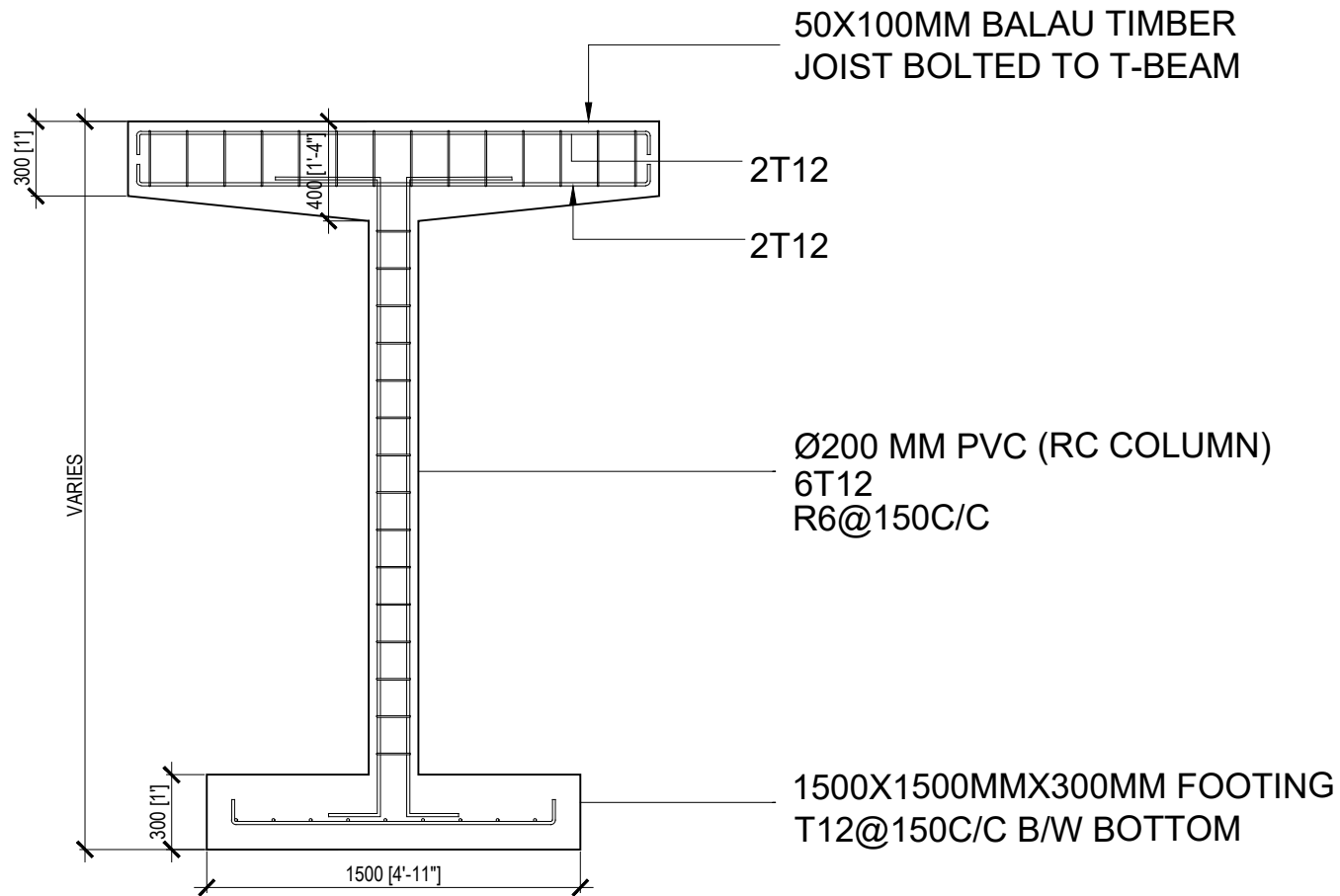
FOUNDATION/COLUMN/BEAM SECTION
