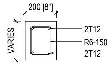
BEAM DETAIL
